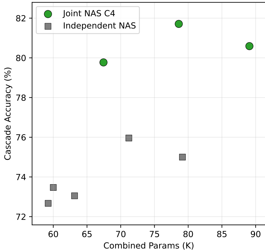
Accuracy vs Model Size at Threshold 0.70
