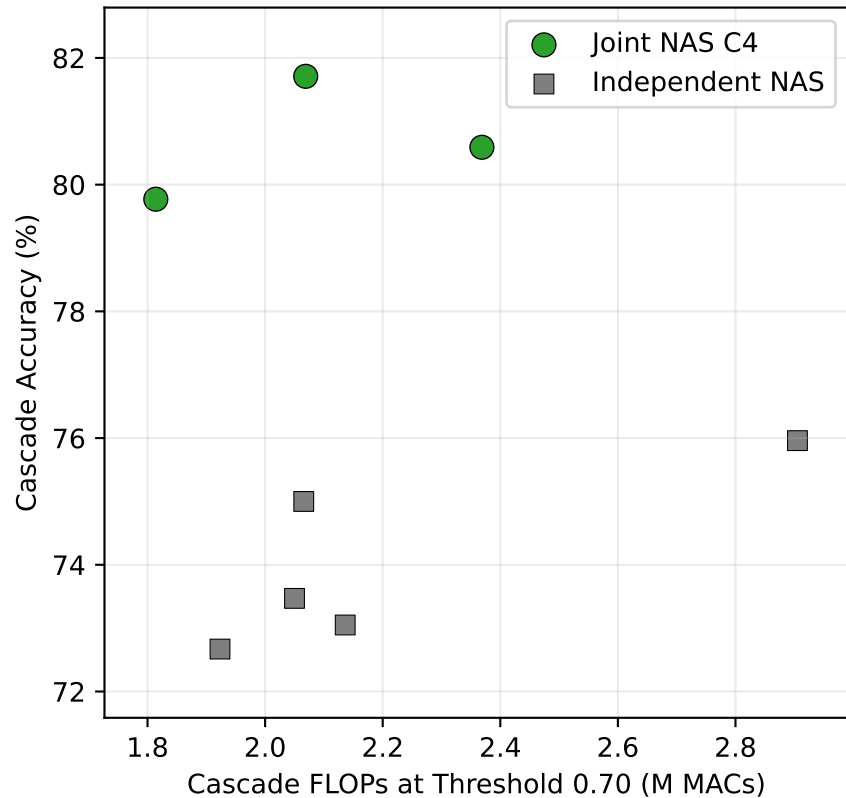
Accuracy vs Compute at Threshold 0.70
