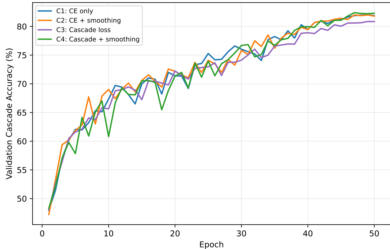
C1-C4 Training Curve Overlay - Architecture 3
