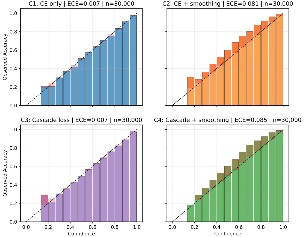
Fig. 11. Confidence-accuracy reliability diagrams for the C1-C4 retraining variants. The figure complements the ECE and routing-error summaries by showing where each variant is under- or over-confident across confidence bins.
