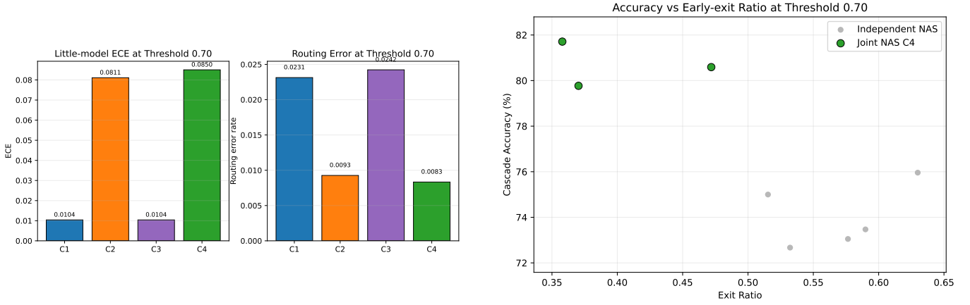
Fig. 6. Routing and confidence behaviour at \tau = 0.70 . The left panel shows little-model ECE and routing error for the C1-C4 retraining variants, while the right panel relates cascade accuracy to early-exit ratio for joint and independent cascades. These metrics show why exit ratio must be interpreted together with confidence quality and accuracy.
