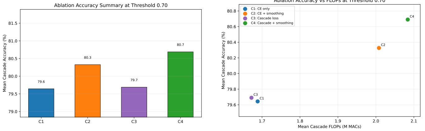
Fig. 5. Retraining-loss ablation for the three selected joint architectures at \tau = 0.70 . C1 uses CE, C2 uses CE with label smoothing, C3 uses the cascade-aware loss, and C4 combines cascade-aware loss with label smoothing. The ablation shows that C3 slightly improves the CE operating point, while the strongest average accuracy and lowest routing error are associated with the smoothed variants.
