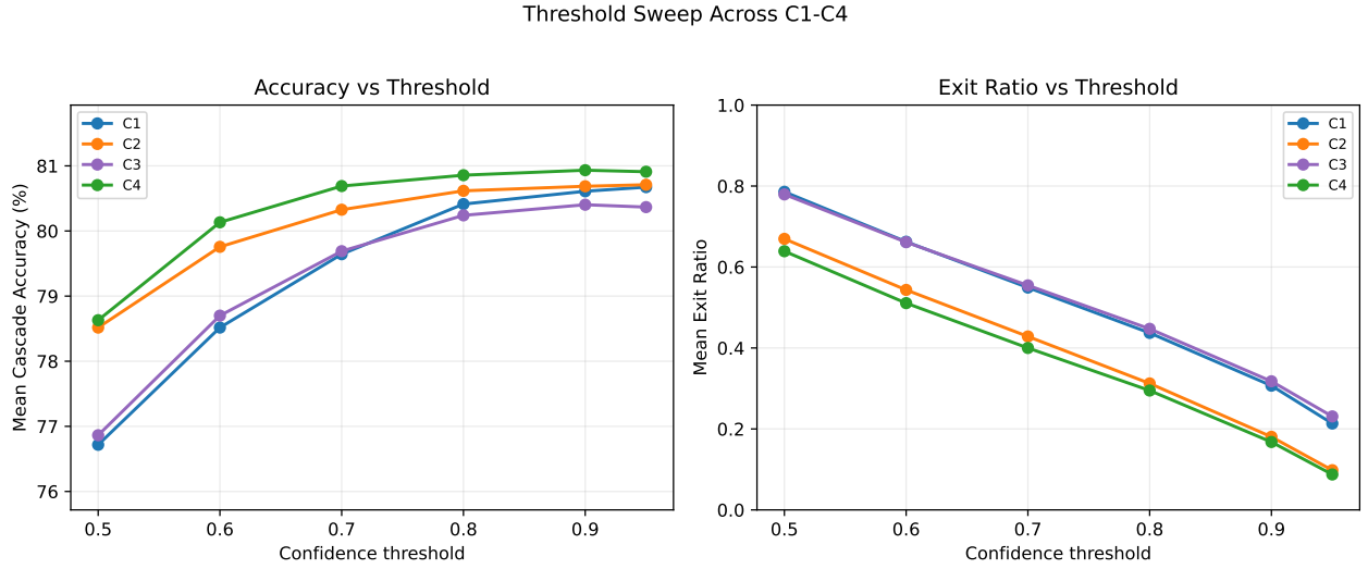
Fig. 7. Threshold sweep for the C1-C4 retraining variants. Increasing the confidence threshold reduces the early-exit ratio and generally improves cascade accuracy by deferring more samples to the big model. Lower thresholds produce cheaper, more exit-heavy cascades, while higher thresholds approach big-model behaviour. The cascade-aware variants, C3 and C4, were trained with the same threshold through a soft routing term, so their sweep also shows how that training objective transfers when the inference threshold is moved away from \tau = 0.70 .
