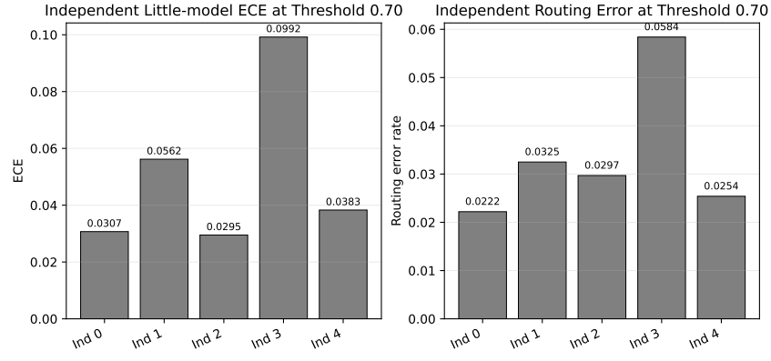
Fig. 10. Independent-baseline routing diagnostics at \tau = 0.70 . The independent baseline can have lower ECE than some joint variants, but it still has lower cascade accuracy, showing that calibration alone is not sufficient to explain the final trade-off.
