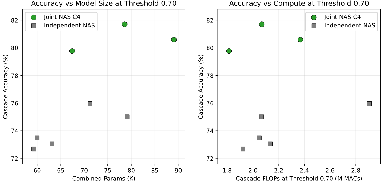
Fig. 4. Final retrained high-accuracy joint cascades compared with independently searched cascades at the fixed operating threshold \tau = 0.70 . The plot uses the C4 retraining condition to show the high-accuracy end of the joint ablation, not to define C4 as the single canonical joint result. The left panel compares combined parameter count against cascade accuracy, while the right panel compares expected cascade FLOPs against cascade accuracy.
