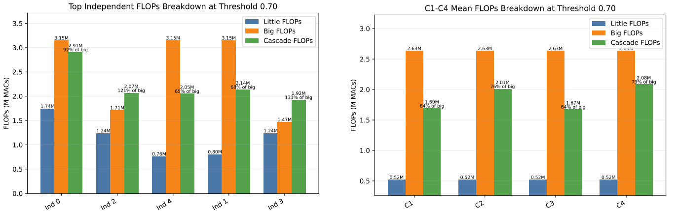
Fig. 9. FLOPs breakdown at \tau = 0.70 . The independent baseline and joint variants use different selected architecture pairs, while the C1-C4 joint ablations use the same selected architectures. Changes in expected cascade FLOPs within the joint ablation therefore mainly reflect differences in exit ratio caused by the retraining objective.
