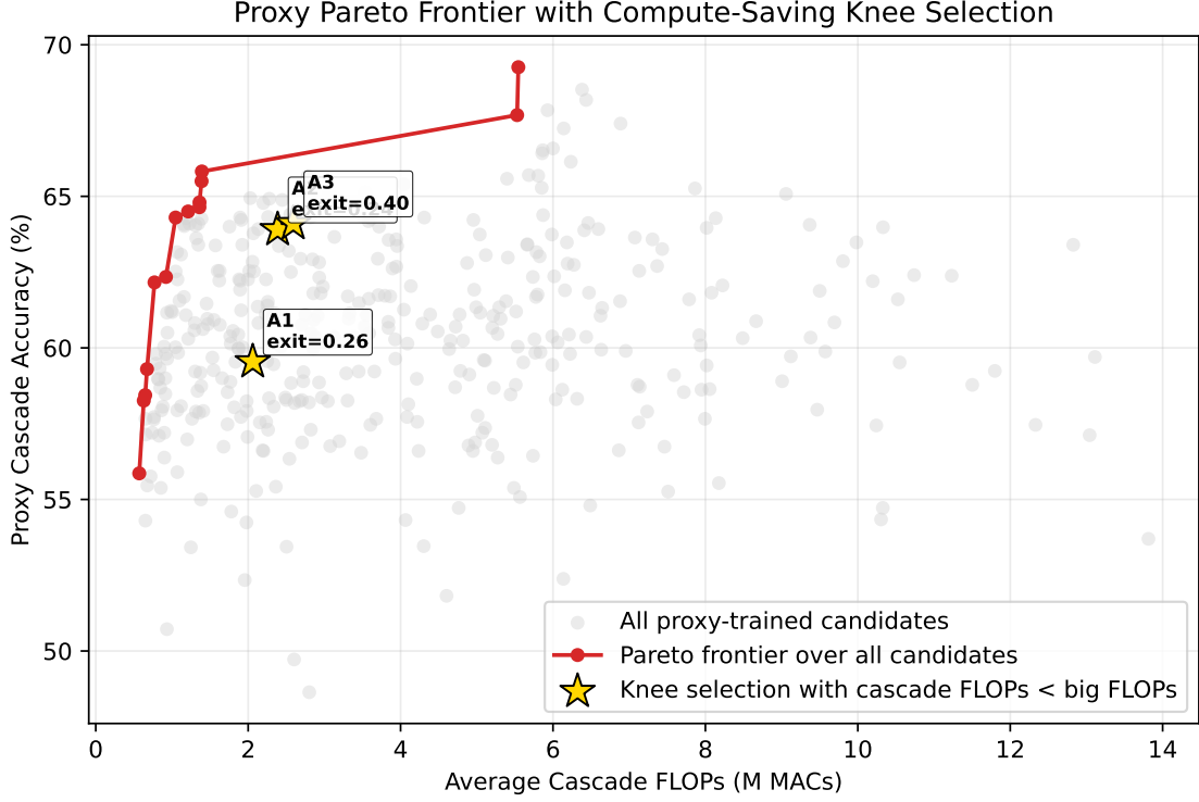
Fig. 8. Proxy Pareto frontier used to select joint architectures for full retraining. The selected candidates are chosen from the compute-saving knee region after feasibility checks and the constraint F_{\text{cascade}} < F_b , not simply by taking the three highest proxy-accuracy points. The figure therefore documents the selection heuristic; final claims are based on fully retrained test-set results rather than the 5-epoch proxy scores.
