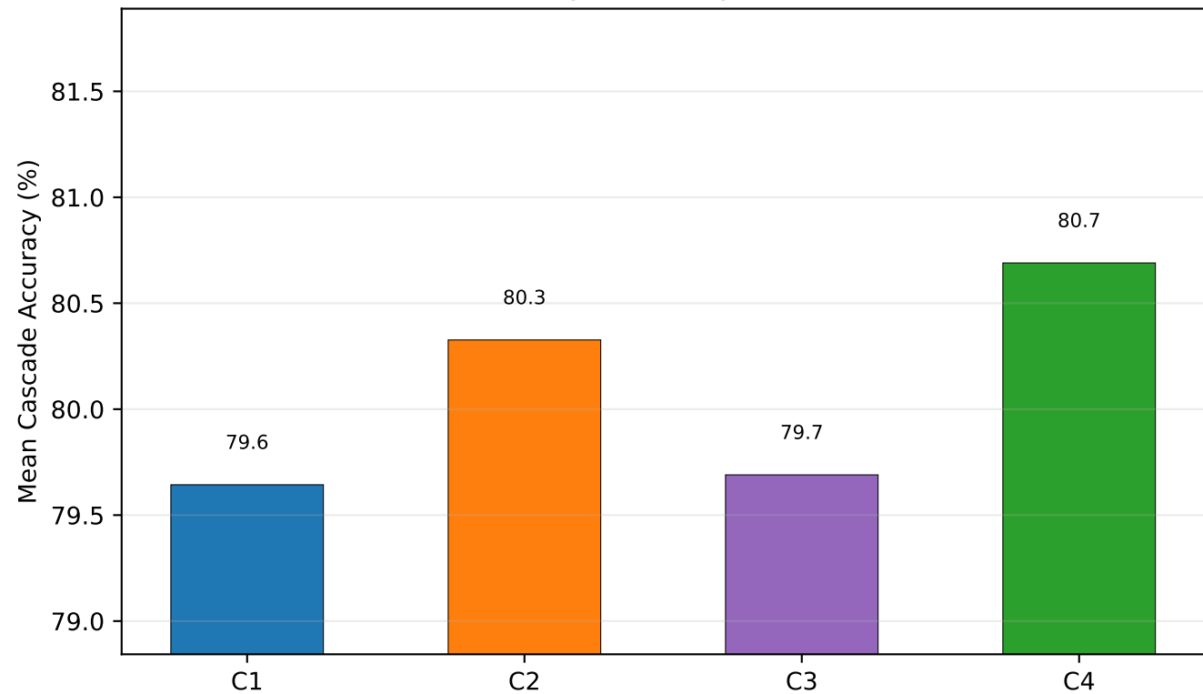
Ablation Accuracy Summary at Threshold 0.70
