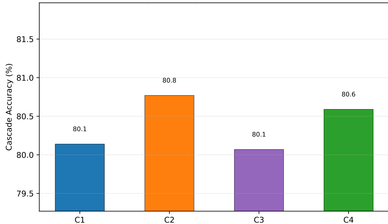
Ablation Accuracy Summary at Threshold 0.70 - Architecture 3
