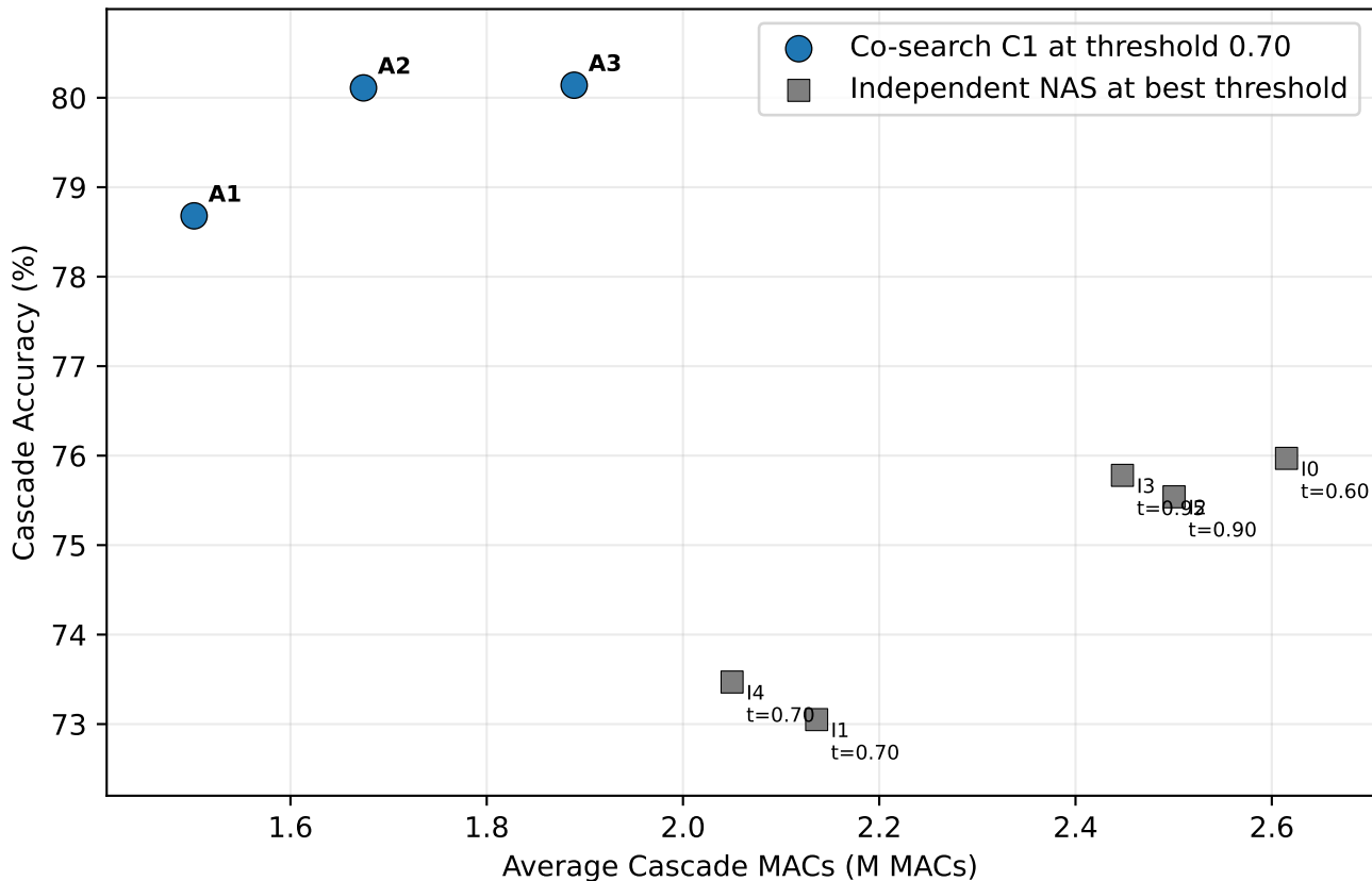
C1 Co-search vs Independent NAS with Best Independent Threshold
