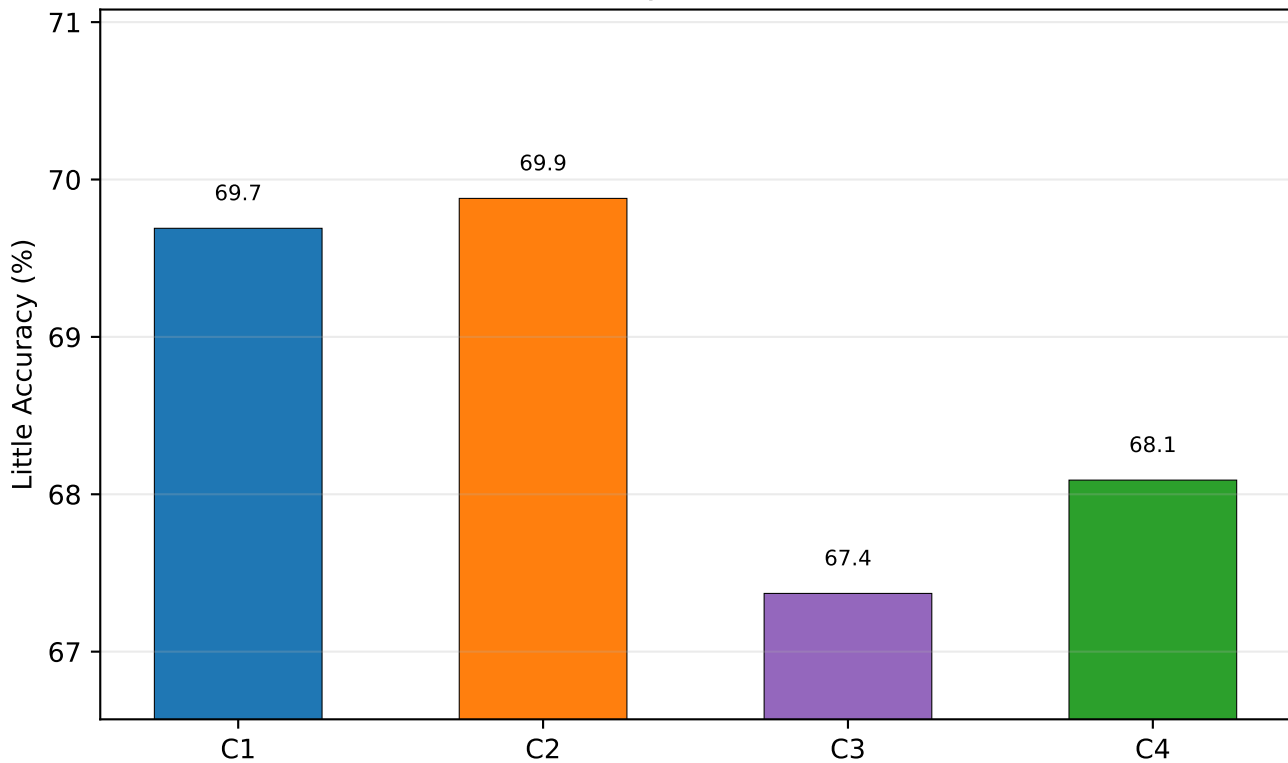
Ablation Little-model Accuracy at Threshold 0.70 - Architecture 1
