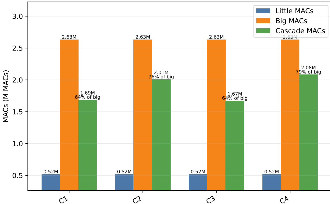
C1-C4 Mean MACs Breakdown at Threshold 0.70
