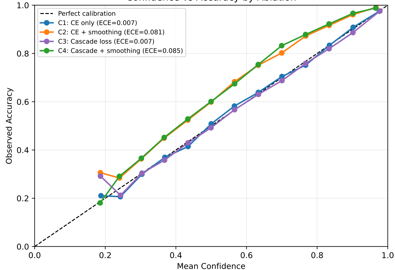
Confidence vs Accuracy by Ablation
