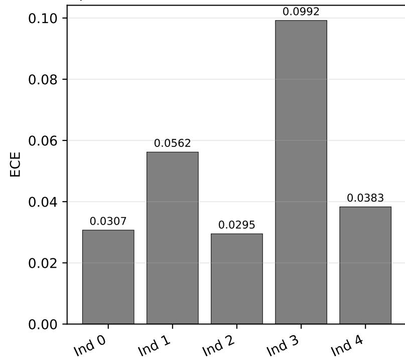
Independent Little-model ECE at Threshold 0.70
