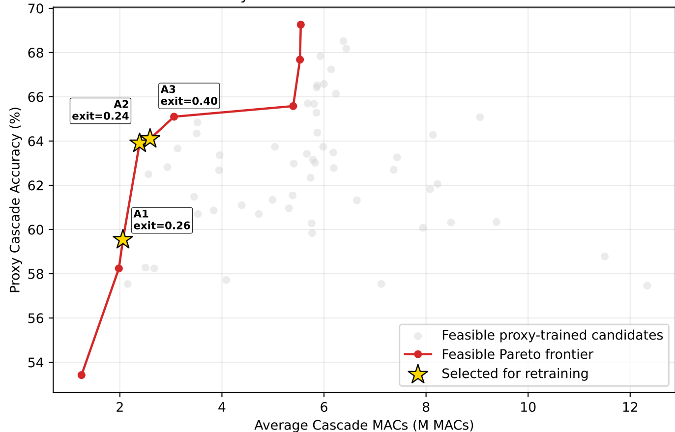
Feasible Proxy Pareto Frontier with Selected Architectures
