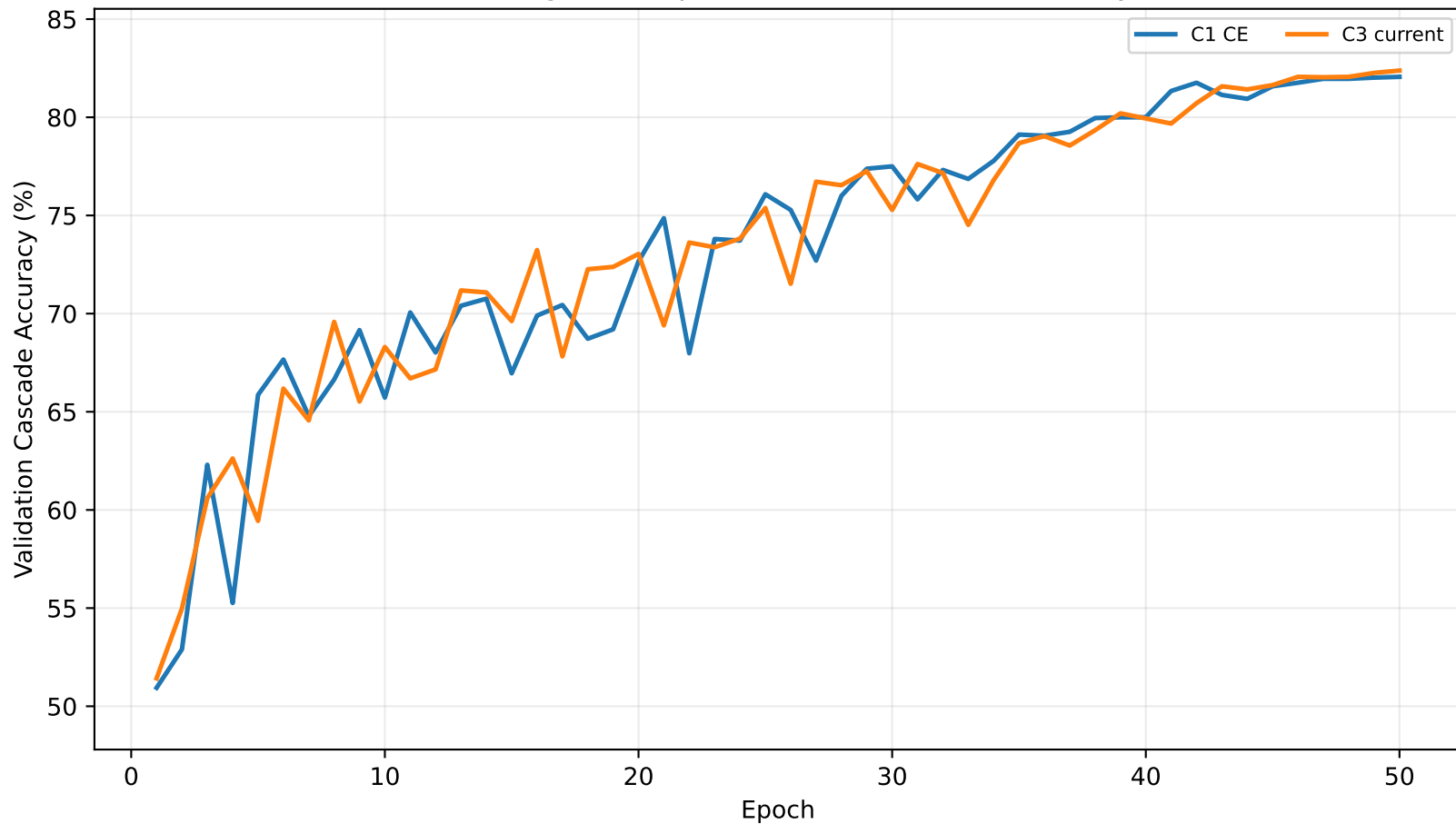
C1 vs C3 Weight Sweep: Validation Cascade Accuracy (A2)
