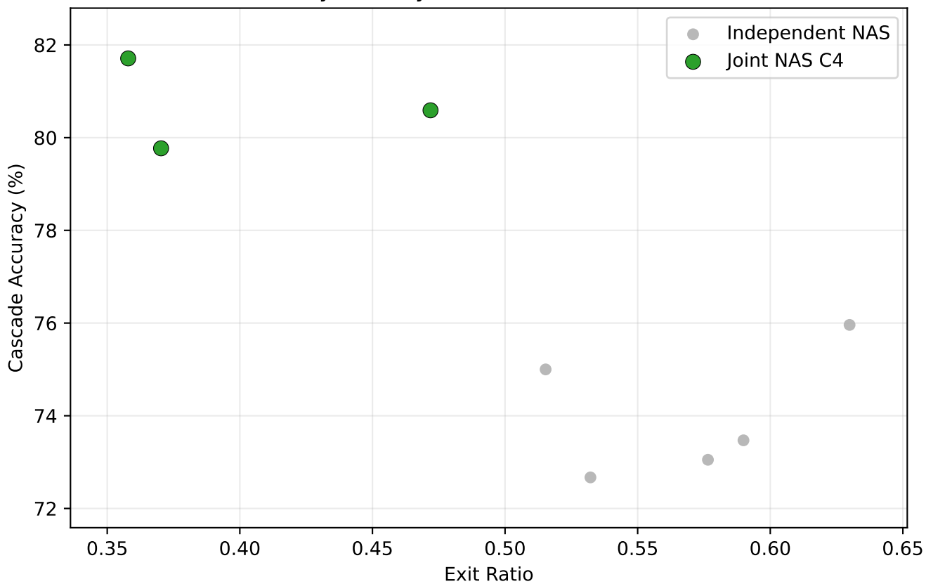
Accuracy vs Early-exit Ratio at Threshold 0.70
