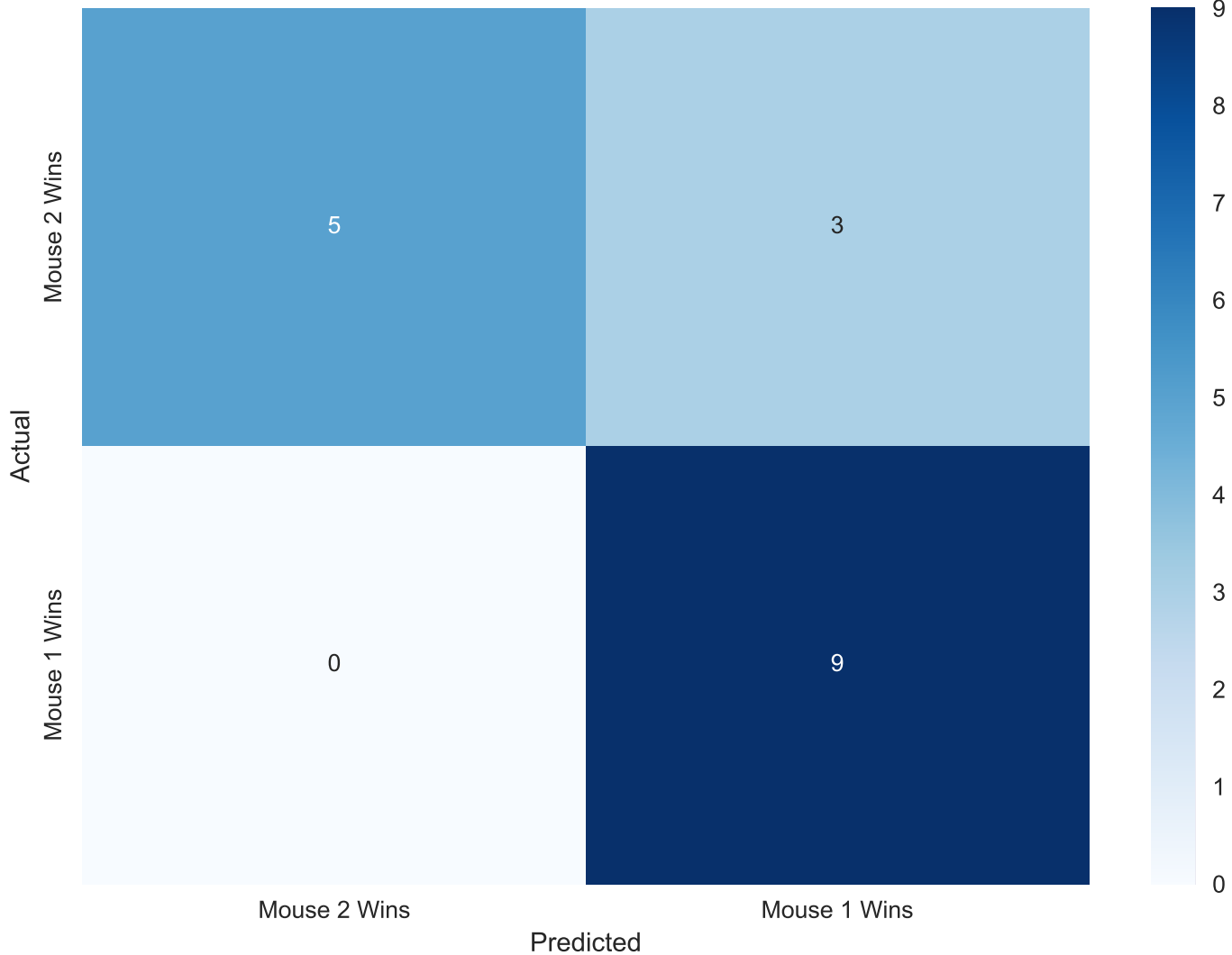
Confusion Matrix - Epoch 18
