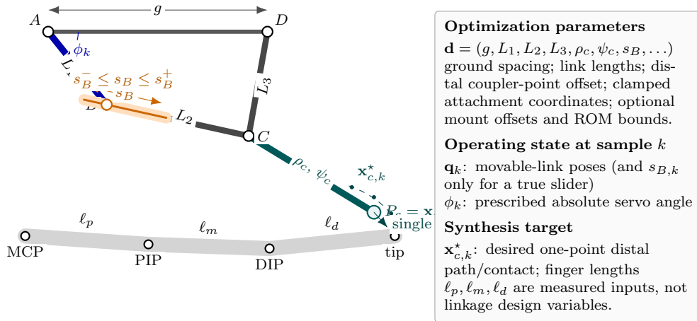
Figure 2: Reference-inspired candidate architecture for one digit and the principal geometry exposed to trajectory optimization. The orange attachment is either clamped at design coordinate s_B or promoted to a bounded runtime slider; those are different mathematical models.
