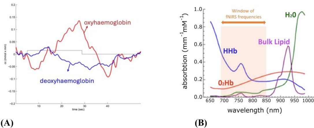
Figure 2. (A) Canonical HRF in a newborn (Issard & Gervain, 2018) (B) Differential light absorption spectra of HbO and HbR in NIR range (Kumar et al., 2017)
