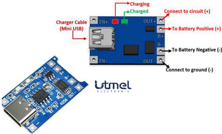
TP4056 Pinout
