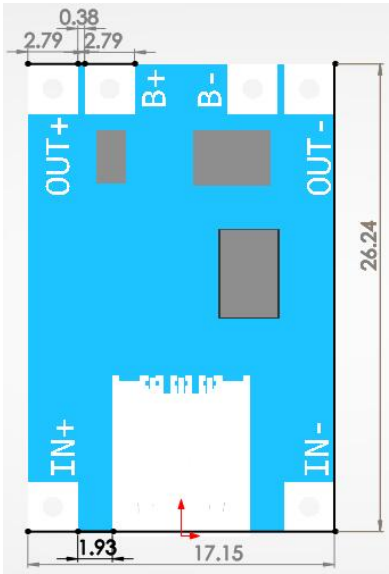
TP4056 Dimension
