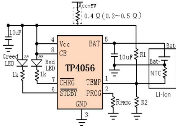
TP4056 Application Circuit
