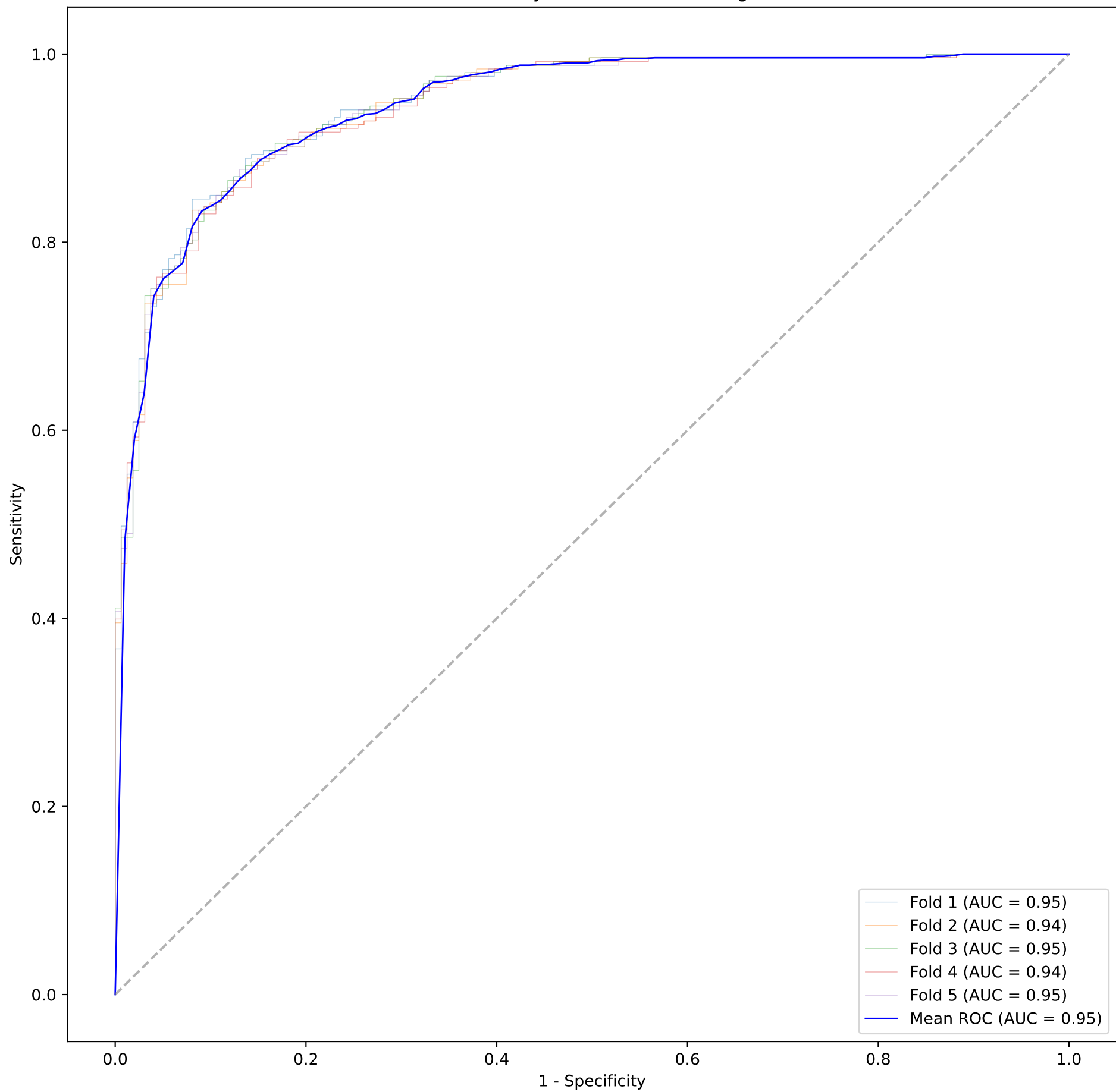
Validation Set ROC by Fold-wise Soft Voting Ensemble
