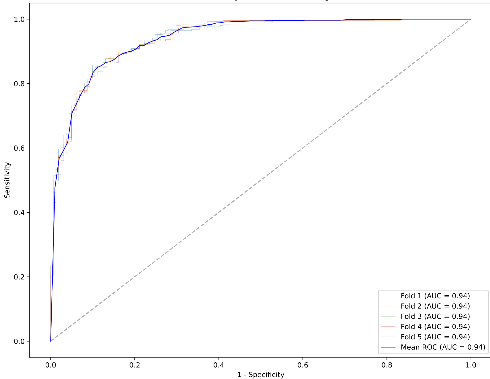
Validation Set ROC by Fold-wise Soft Voting Ensemble
