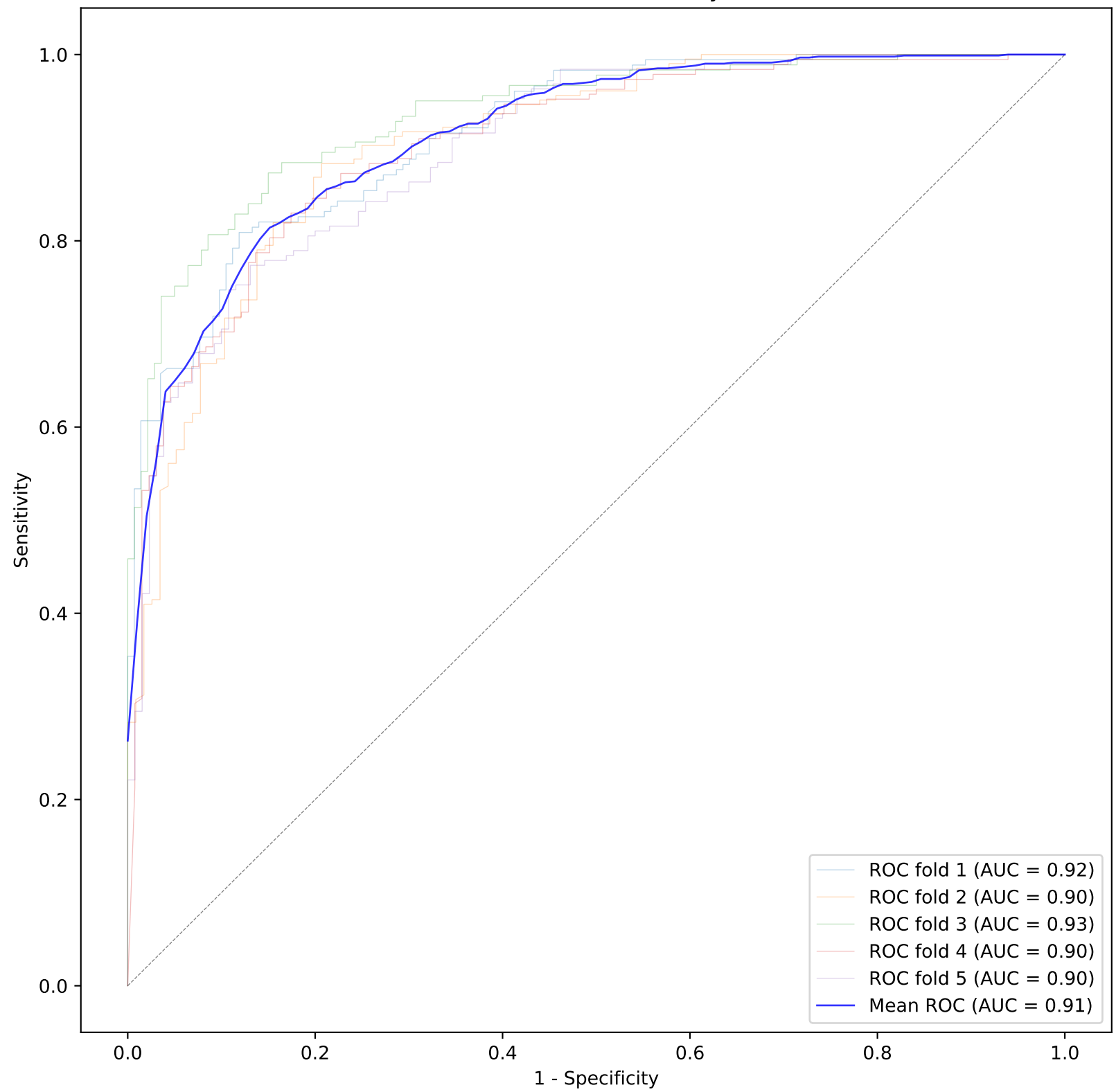
ROC Curve for Naive Bayes
