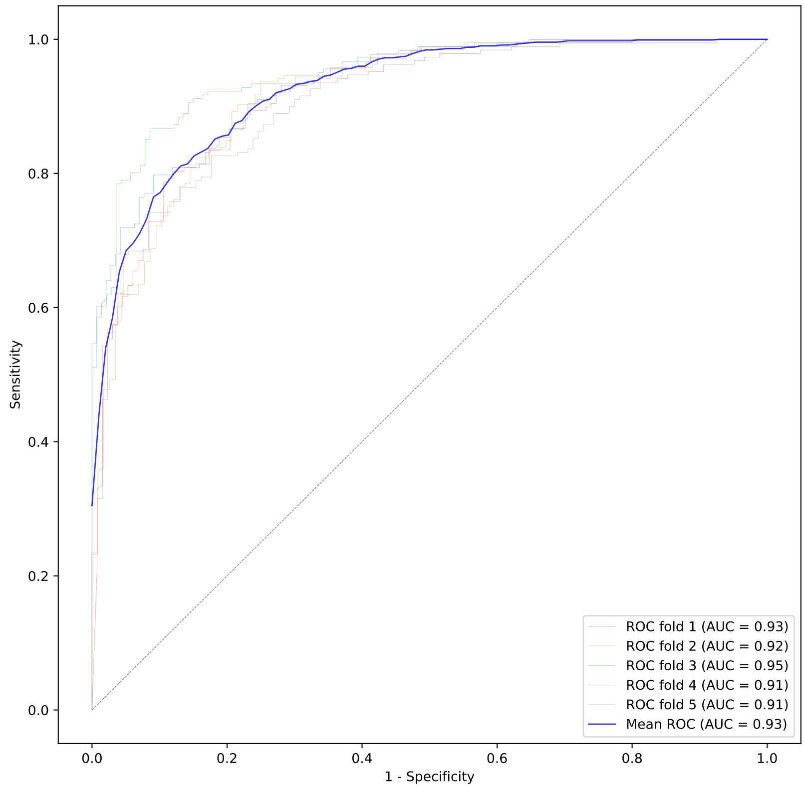
ROC Curve for SVM
