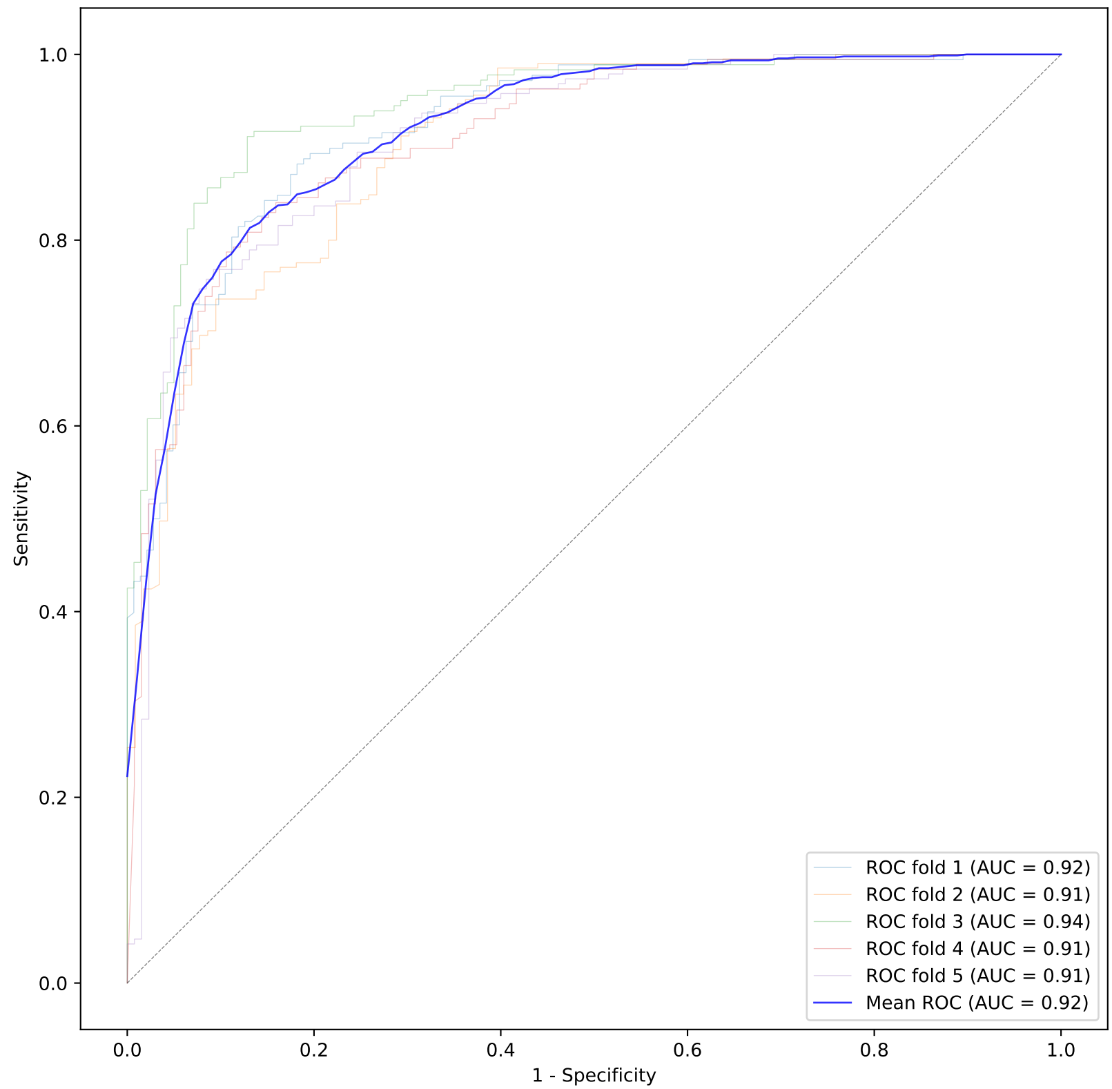
ROC Curve for Random Forest
