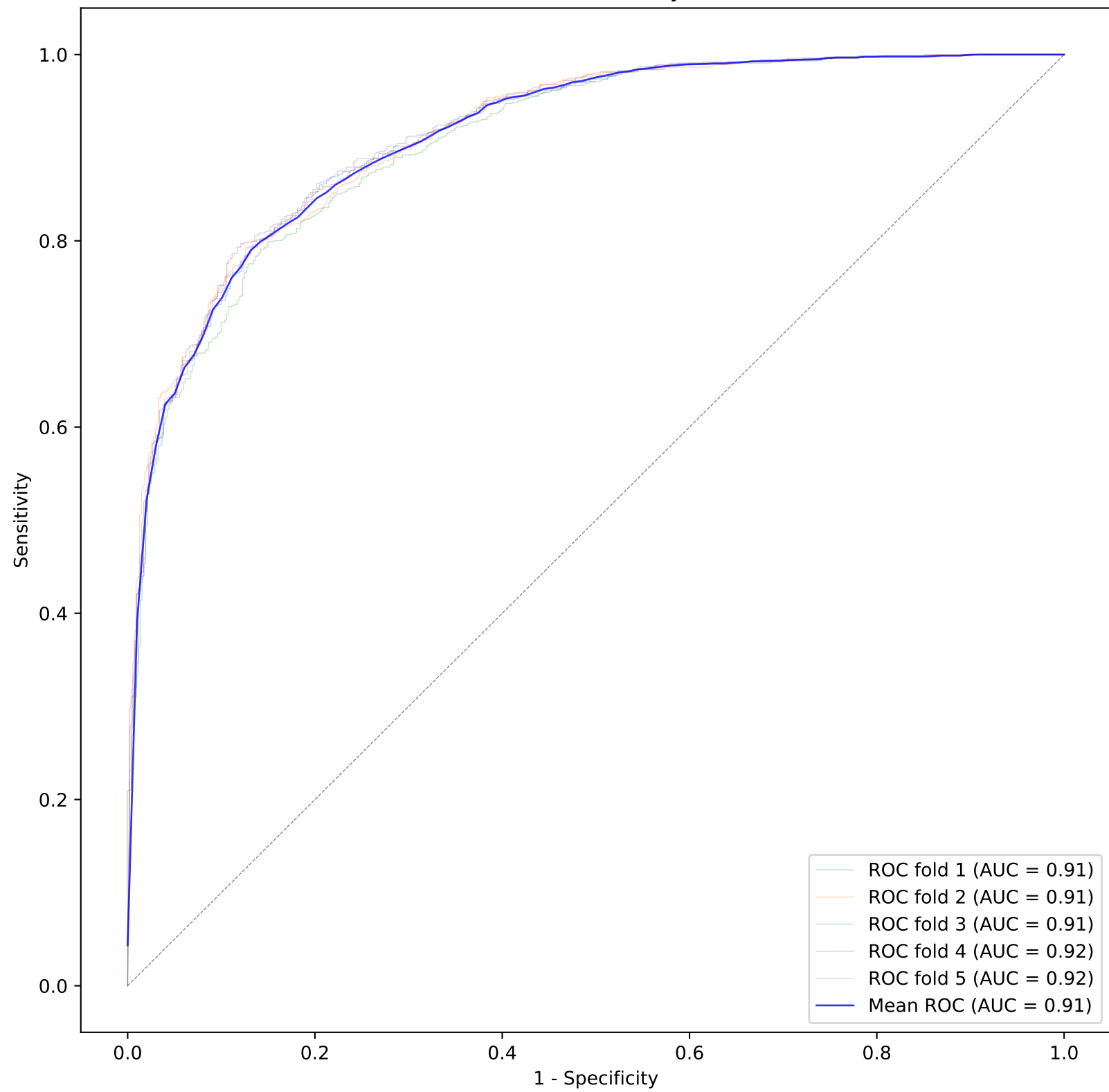
ROC Curve for Naive Bayes (Train)
