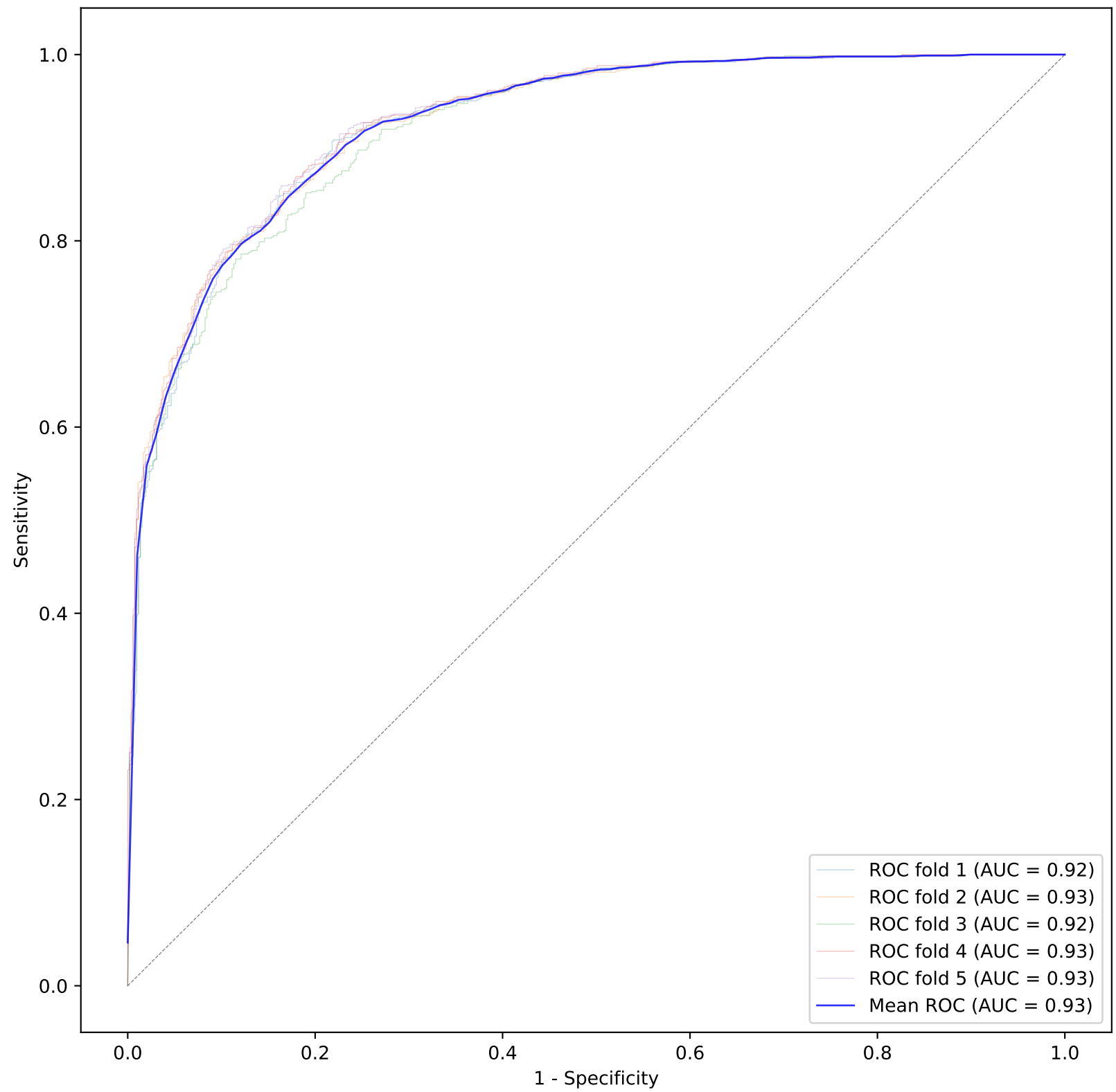
ROC Curve for SVM (Train)
