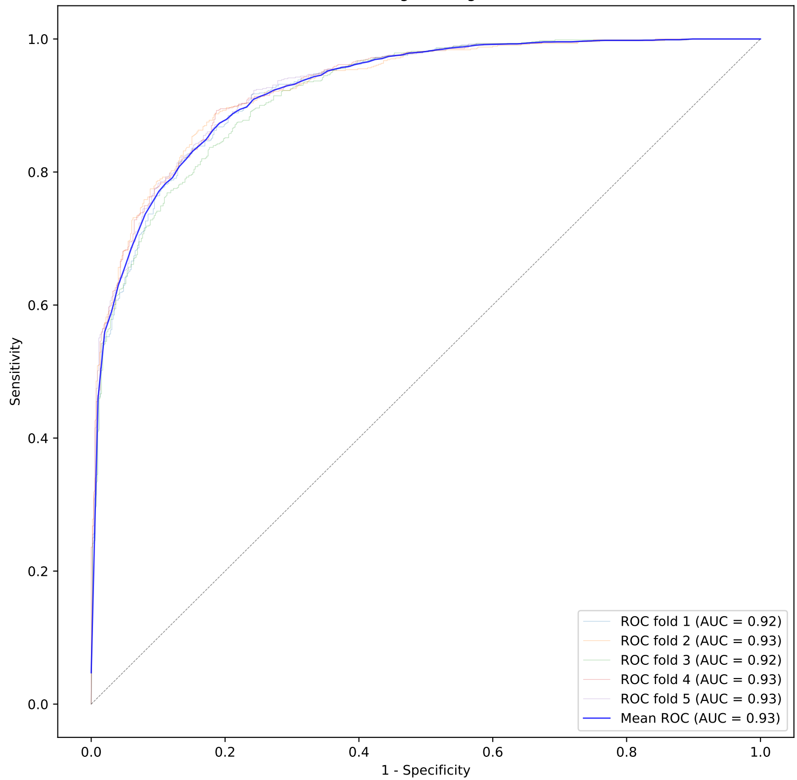
ROC Curve for Logistic Regression (Train)
