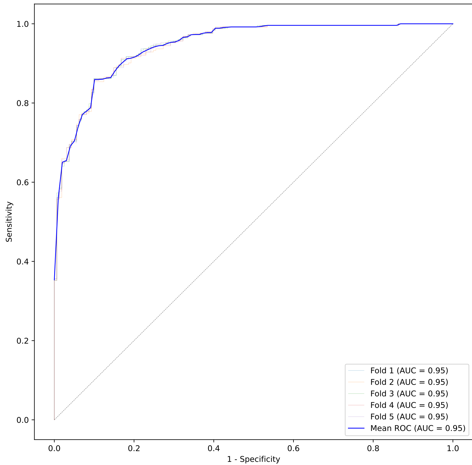
ROC Curve for SVM
