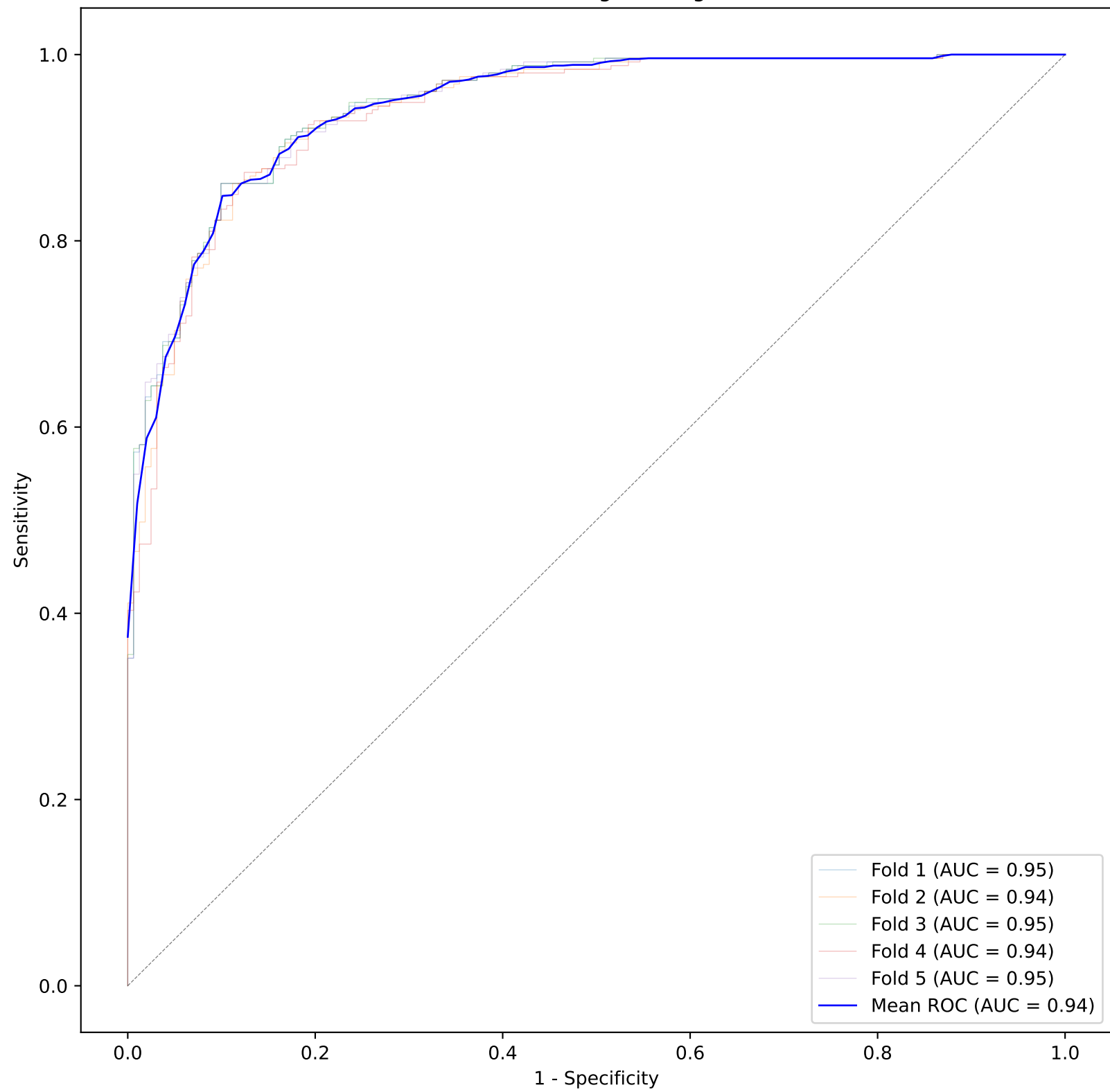
ROC Curve for Logistic Regression
