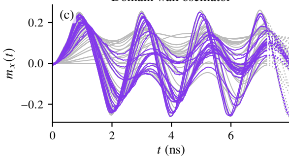
Domain wall oscillator
