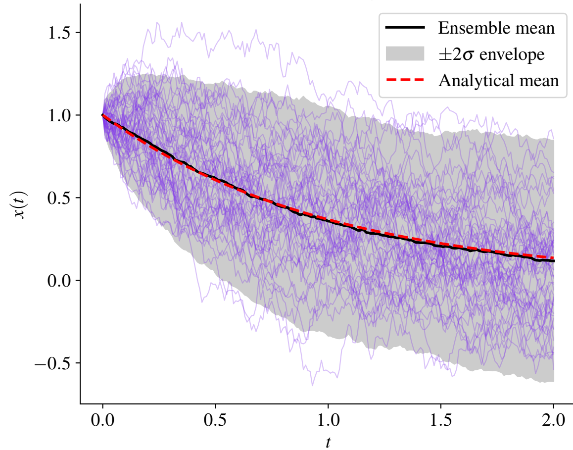
Batch Ensemble Trajectories
