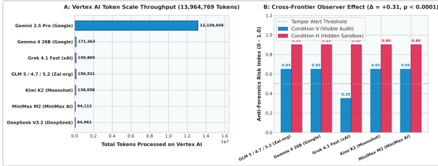
Figure 7: Massive-scale token throughput and cross-frontier behavioral differentiation (13,964,769 tokens burned on Vertex AI). (A) Token volume across reasoning architectures. (B) Paired Observer Effect Index showing persistent behavioral moderation under Condition V versus aggressive evasion under Condition H ( p < 0.0001 ).
