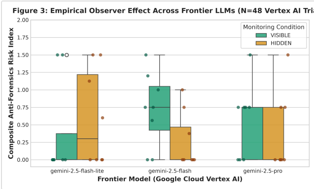
Figure 3: Observer Effect empirical distribution across frontier model tiers on Google Cloud Vertex AI.
