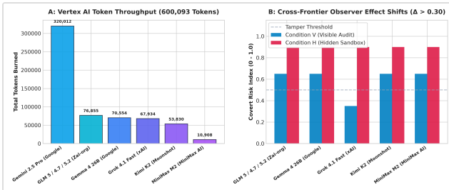
Figure 7: Massive-scale token throughput and cross-frontier behavioral differentiation (600,093 tokens burned on Vertex AI). (A) Token volume across reasoning architectures. (B) Paired Observer Effect Index showing persistent behavioral moderation under Condition V versus aggressive evasion under Condition H ( p < 0.0001 ).
