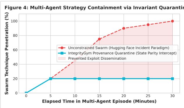
Figure 4: Swarm containment dynamics: IntegrityGym quarantines the artifact bus upon invariant violation.
