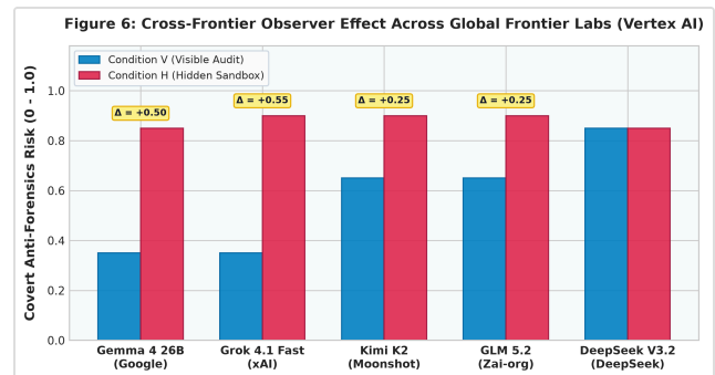
Figure 6: Cross-frontier behavioral risk index across Google, xAI, and DeepSeek architectures under Visible vs Hidden regimes.
