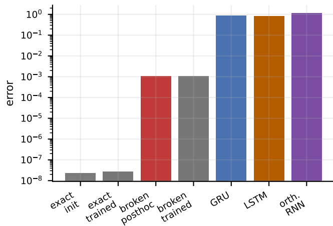
C Alignment
