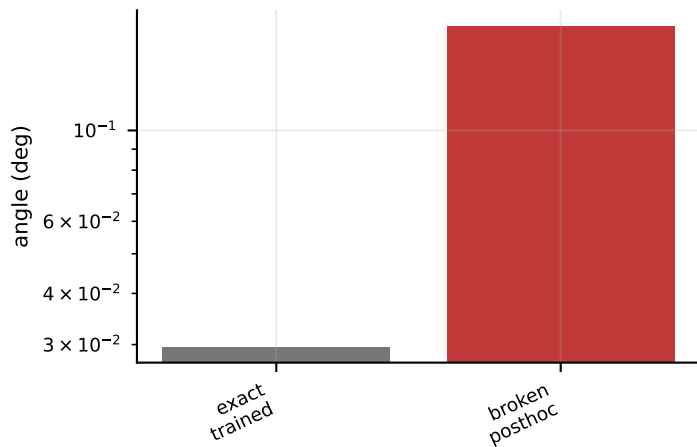
C Alignment
