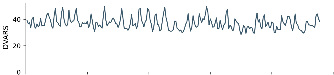
DVARS — pre-denoising (raw fMRIPrep)
