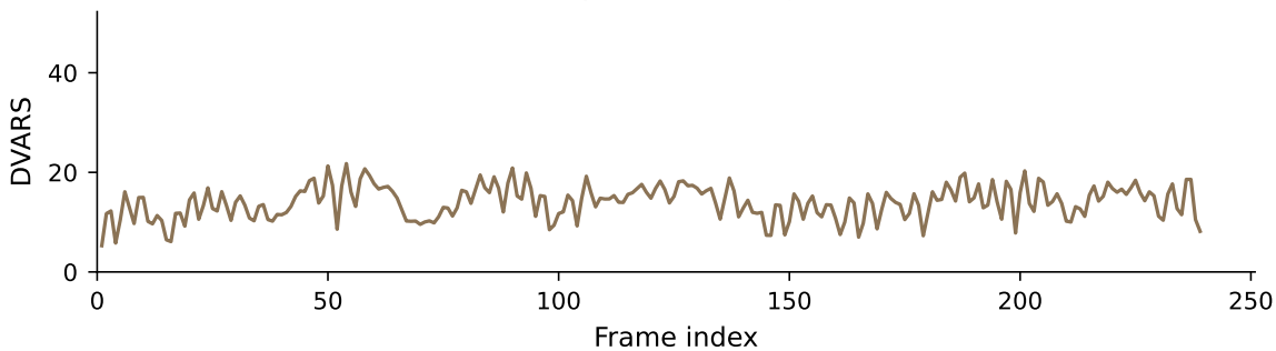
DVARS — post-denoising (+GSR)
