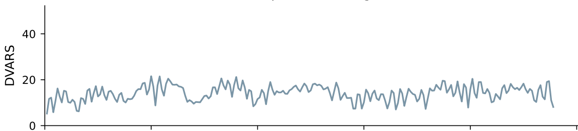
DVARS — post-denoising (-GSR)
