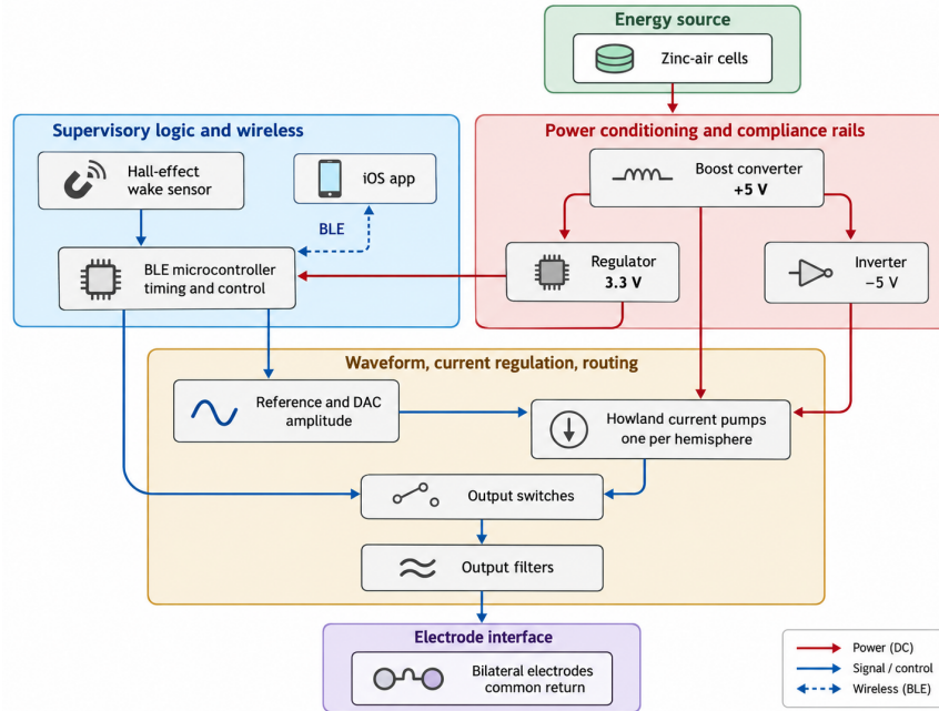
Figure 1. FLEX-DBS architecture. Functional blocks used to describe rodent stimulators, as implemented in FLEX-DBS. Zinc-air cells feed a boost converter that generates the +5 V rail; an inverter derives -5 V, and a regulator derives 3.3 V for the BLE microcontroller. The microcontroller sets pulse timing, commands amplitude through a reference and DAC, and controls the output switches. The DAC drives two Howland current pumps on \pm 5 V, one per hemisphere, whose outputs pass through the switches and output filters to bilateral electrodes with a common return. A Hall-effect sensor wakes the device when a magnet is passed over it, and parameters are set from an iOS application over BLE. Components are listed in Table 1.
