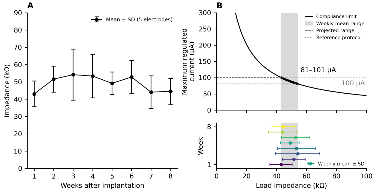
Figure 4. In-vivo electrode impedance and the compliance envelope. (A) Impedance of implanted platinum electrodes from 1 to 8 weeks after implantation, a pulse-derived estimate of the effective load computed as pulse voltage over delivered current with 10 \mu\text{A} , 450 \mu\text{s} pulses (five readings averaged per electrode and session). Points show the mean \pm SD across five electrodes from three mice; three of eight implanted electrodes were excluded (Section 3.2). (B) Top: largest regulated current of FLEX-DBS as a function of load impedance, I_{\text{max}} = 4.6 \text{ V}/(|Z| + 2.66 \text{ k}\Omega) , with the swing measured into 47 \text{k}\Omega . The gray band spans the range of weekly mean impedances in (A), 43–54 \text{k}\Omega , and the dashed lines project it to the corresponding current range, 81–101 \mu\text{A} ; the dotted line marks the 100 \mu\text{A} reference protocol. Bottom: weekly mean \pm SD impedance on the same impedance axis, colored from week 1 (bottom) to week 8 (top).
