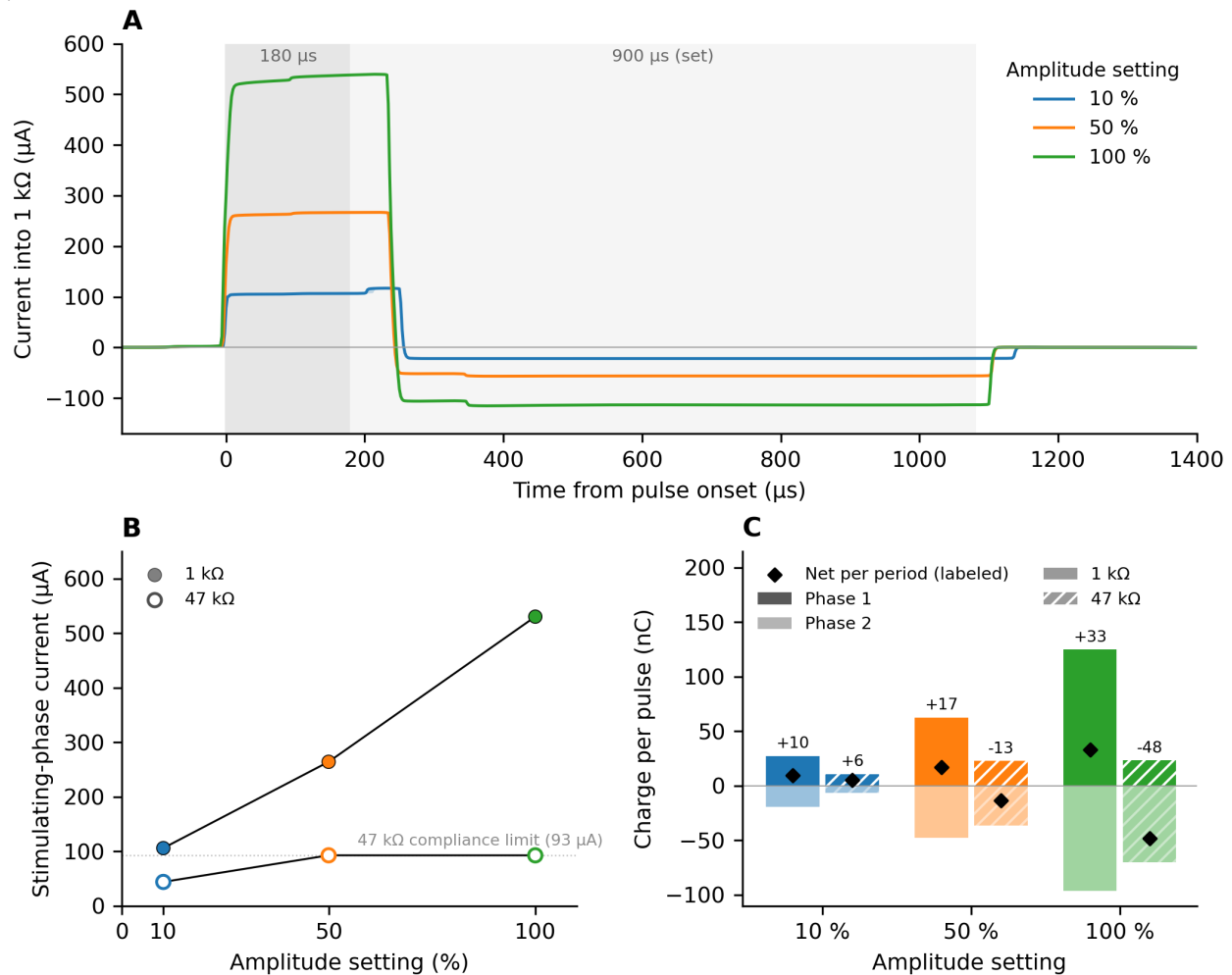
Figure 5. Bench output into 1 k \Omega and 47 k \Omega loads. Both outputs of a FLEX-DBS device (firmware v0.5) were loaded with 1 k \Omega , or with a nominal 47 k \Omega within the in-vivo load range, and one output was recorded at 500 kHz for \sim 11 s at each of three amplitude settings (10, 50 and 100 %; 180 \mu s, 130 Hz). Current is the voltage across the load divided by the load resistance, after a 38 \mu s median filter that removes range-switching artifacts of the meter. (A) Median pulse at each setting into 1 k \Omega (1545–1602 pulses); the 5th–95th percentile band lies within the line width. Shading marks the set stimulating (180 \mu s) and recovery (900 \mu s) phases. (B) Mean plateau current of the stimulating phase against the amplitude setting into 1 k \Omega (filled) and 47 k \Omega (open). The dotted line marks the 92.6 \mu A compliance limit into 47 k \Omega ; the 10 % point at 47 k \Omega is reduced by slow edges. (C) Charge in each phase of the median pulse at 1 k \Omega (solid) and 47 k \Omega (hatched), and the mean net charge over a full period (labeled; nC, nanocoulombs). At every setting and load the delivered frequency was 142.5 Hz; into 1 k \Omega the stimulating phase lasted 238–254 \mu s and the recovery phase 854–878 \mu s.
