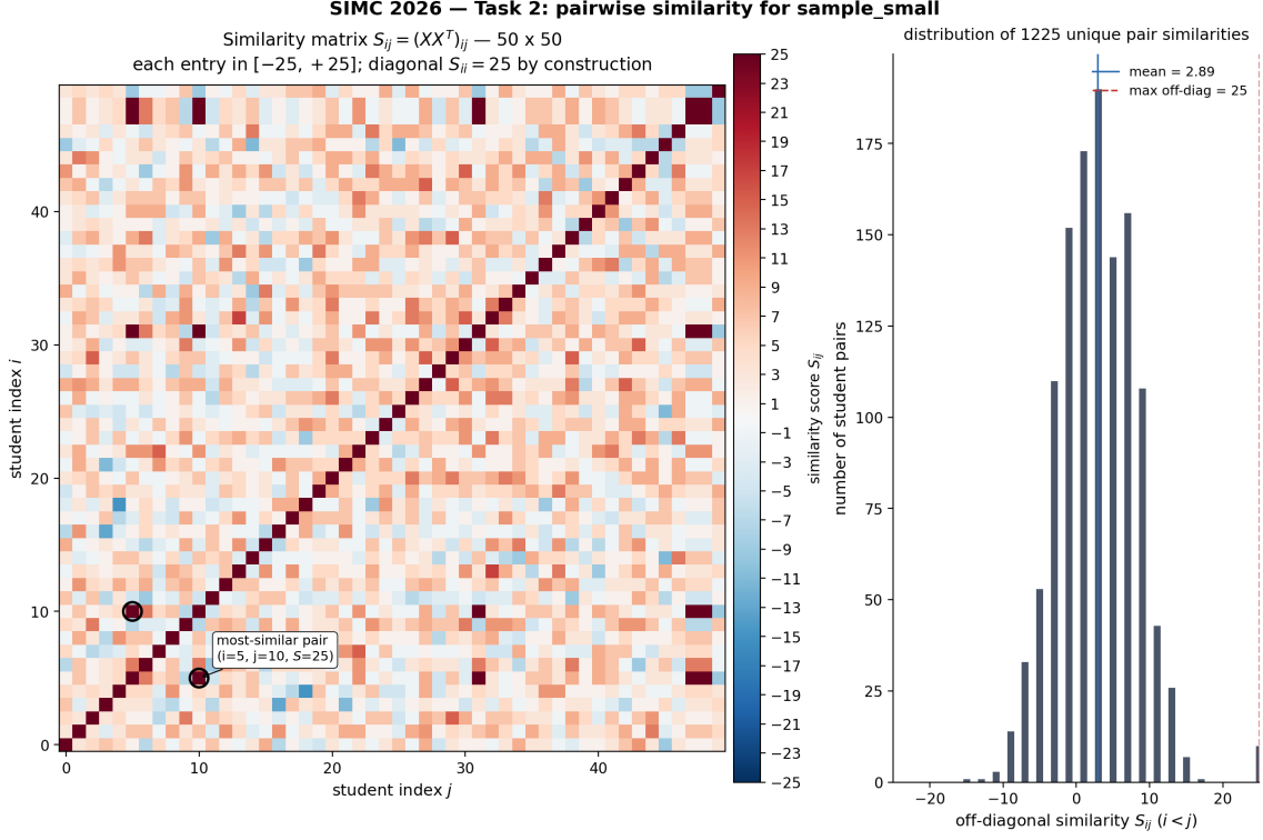
Figure 2: Left: similarity matrix S = XX^T for sample_small . The diagonal S_{ii} = N = 25 is dark red. Right: histogram of off-diagonal S_{ij} with i < j .
