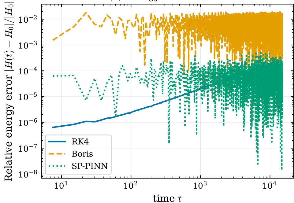
(b) energy conservation
