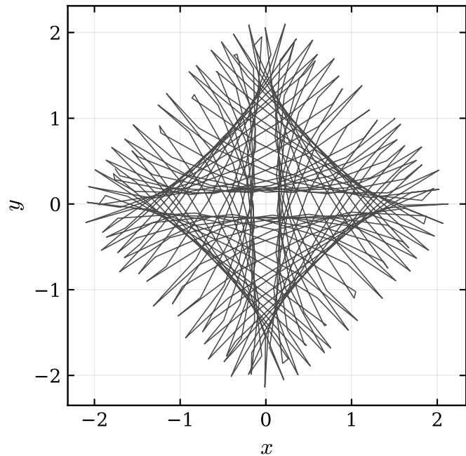
(a) representative orbit
