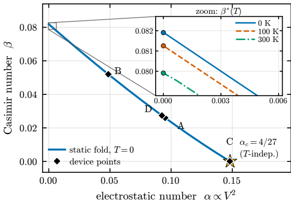
(a) pull-in boundary and device points
