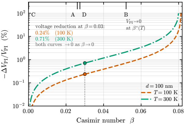
(b) thermal shift of the pull-in voltage
