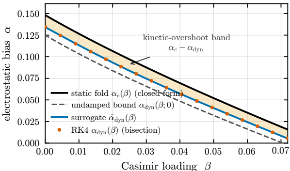
(a) pull-in boundaries at \zeta = 0.1
