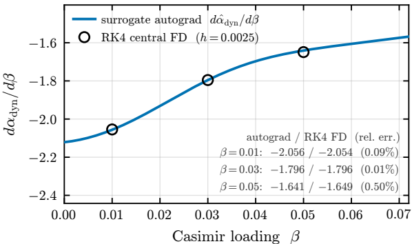
(b) design sensitivity, autograd vs RK4
