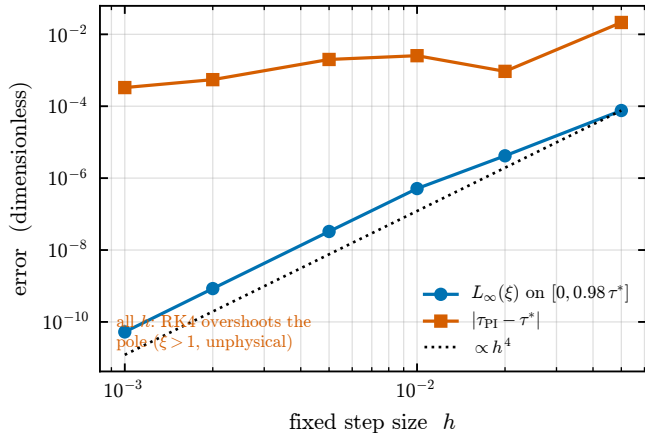
(b) fixed-step RK4 near pull-in
