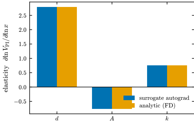
(b) V_{\text{PI}} sensitivities (device A)
