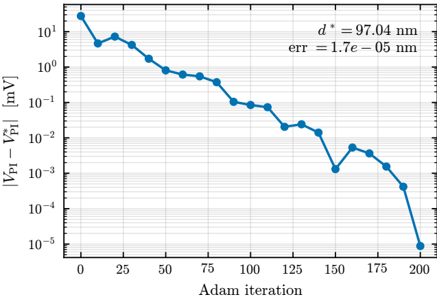
(a) inverse design: gradient descent
