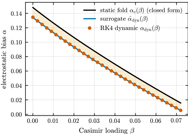
Dynamic vs static pull-in boundary ( \zeta = 0.1 )
