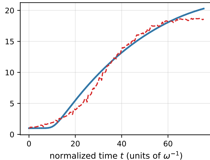
WNL ( a_0 = 8.5 )
