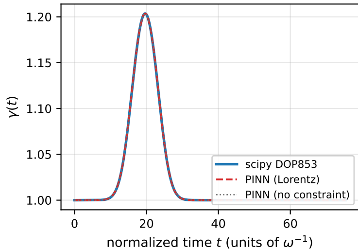
LT ( a_0 = 0.85 )
