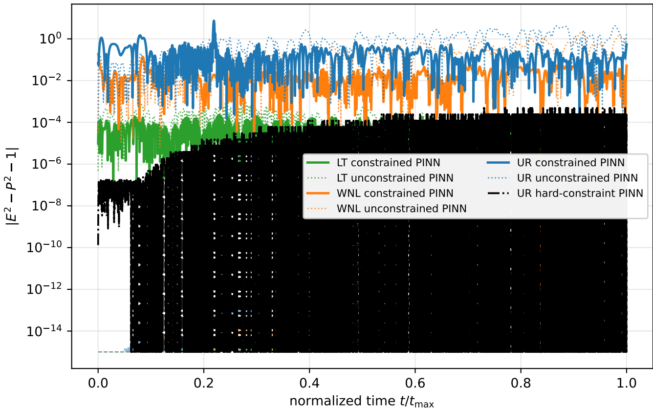
Lorentz invariant conservation error
