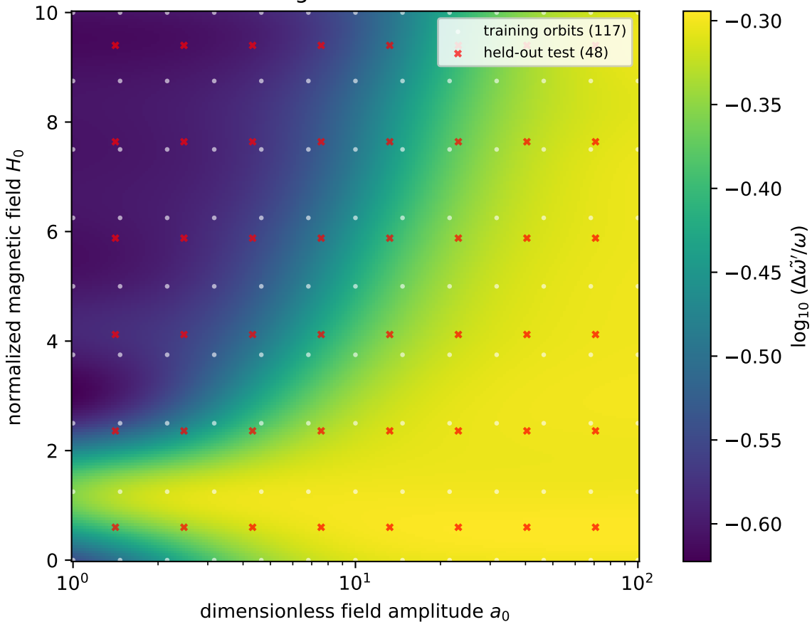
GP surrogate of the simulated linewidth \Delta\tilde{\omega}'/\omega(a_0, H_0) held-out log-RMSE = 5.43e-03
