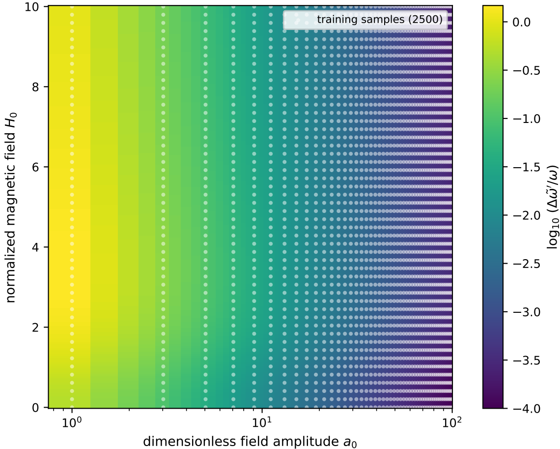
Trained Gaussian-process surrogate \Delta\tilde{\omega}'/\omega(a_0, H_0)
