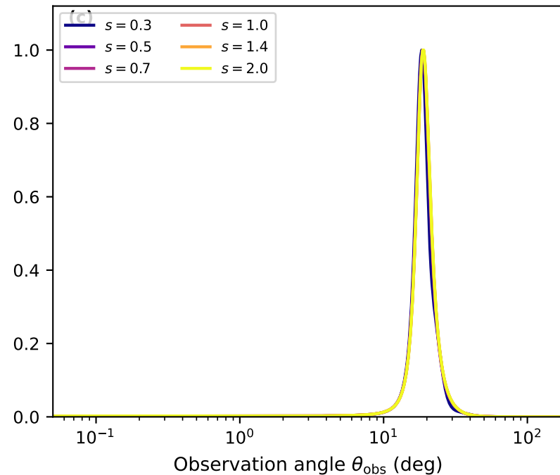
pulse-width series ( L \rightarrow sL , a_0 = 8.5 )
