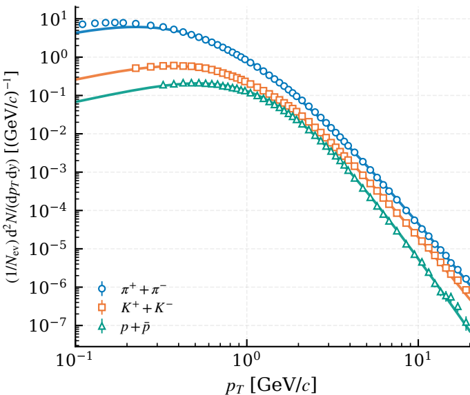
(a) invariant spectra + Tsallis fit
