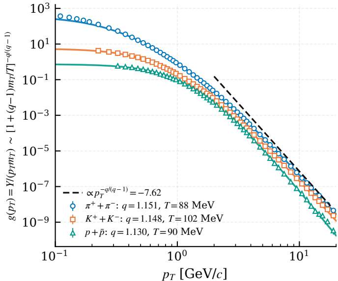
(b) Tsallis function + power-law tail
