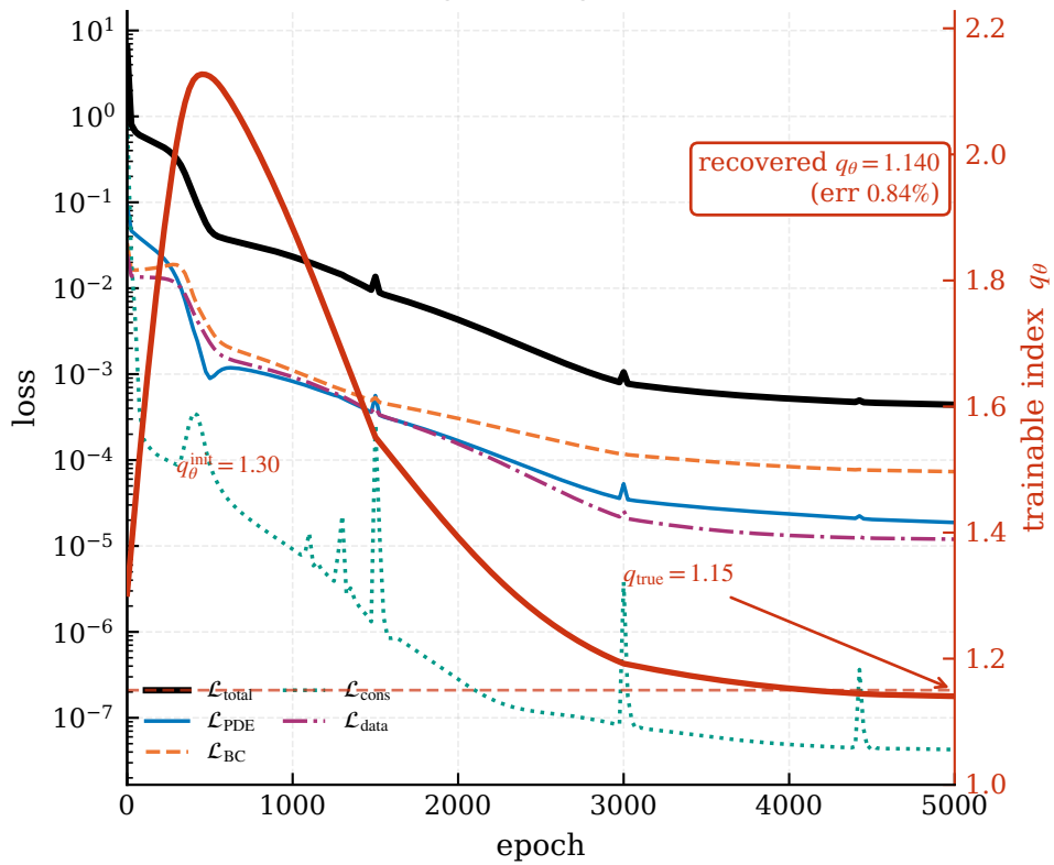
(b) Real training convergence (Adam, CPU)
