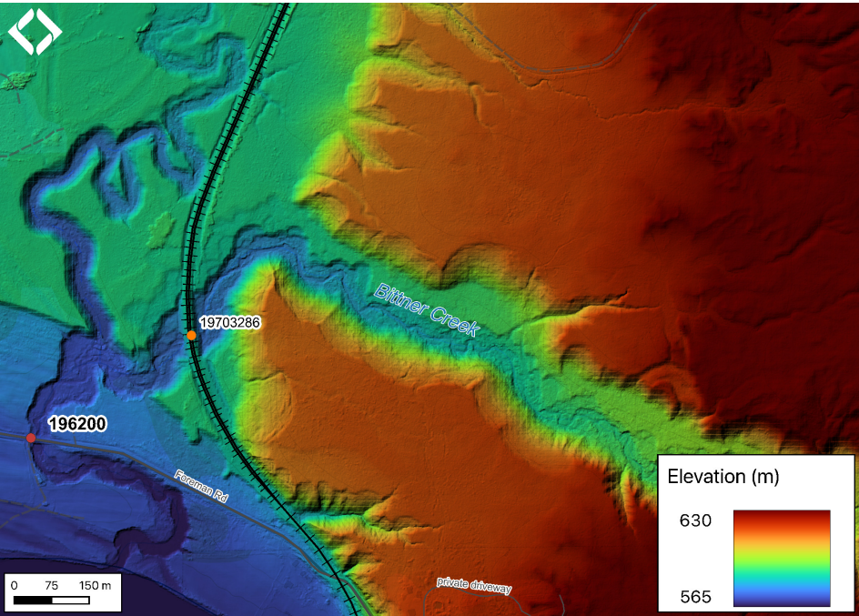
Figure 5.28: Lidar generated digital elevation model of Bittner Creek at Forman Road.
